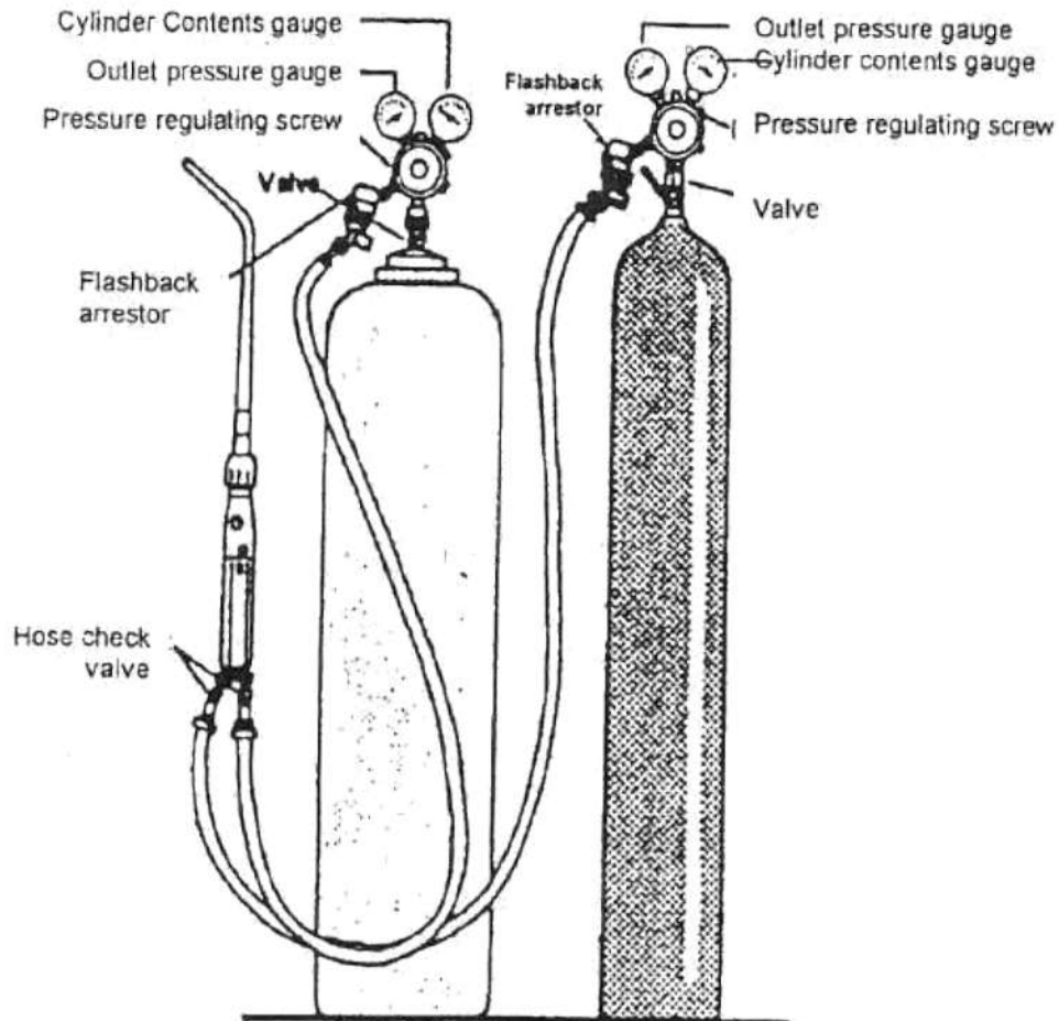
Gas welding equipment showing positions of flashback arrestors and hose check valves
